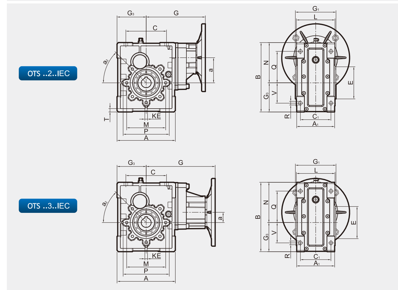
OTS ..IEC外形尺寸 / Outline Dimension
